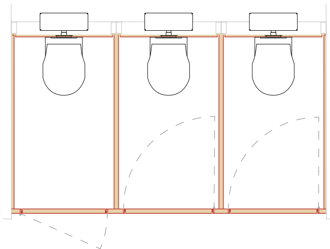
1050.2 Toilet cubicles typical plan
